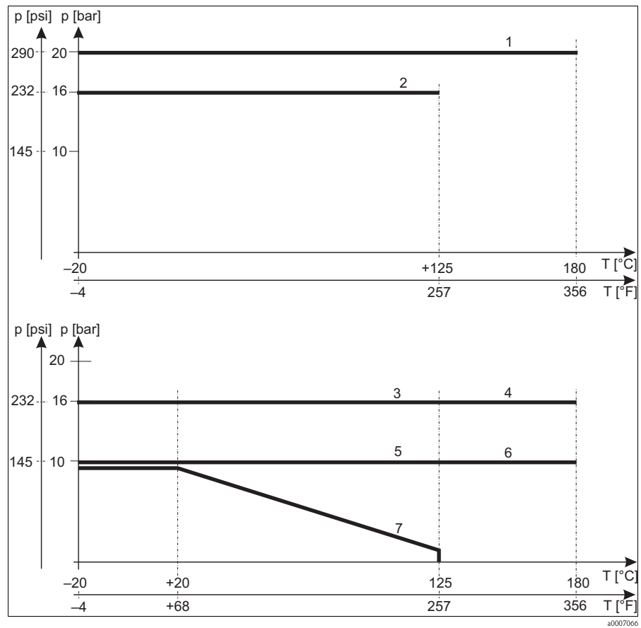
Pressure-temperature diagram (sensor versions, see Ordering information)
