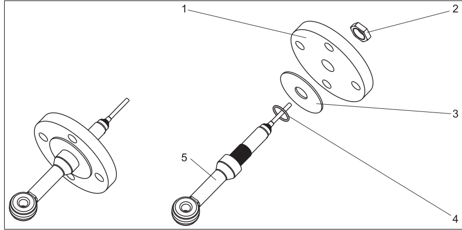
Fixed flange, not in contact with medium (order option "process connection": 5, 6, 7)
