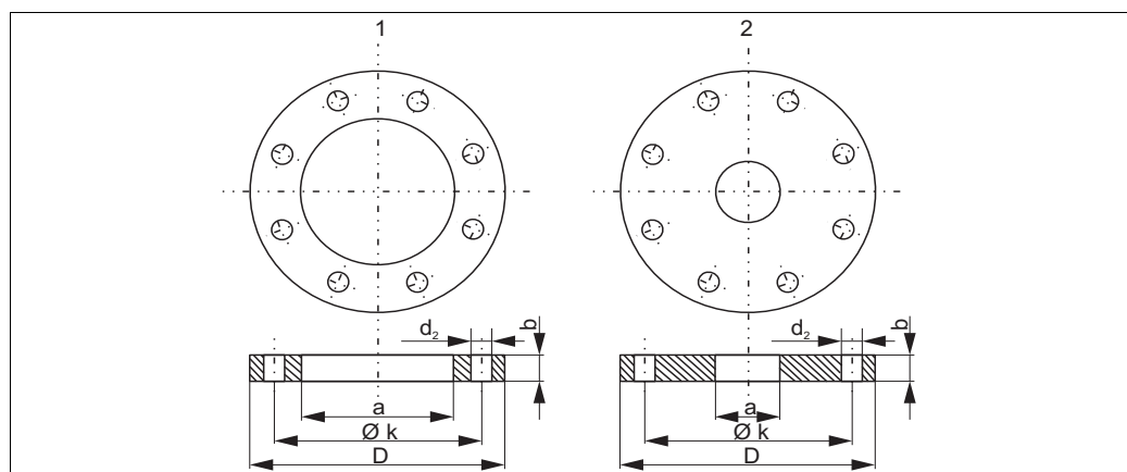
Flange dimensions
