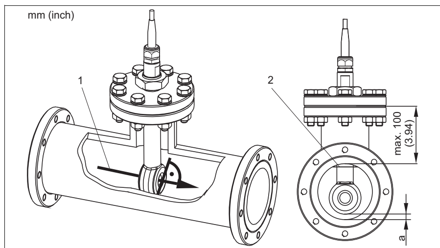
Installation position of the sensor
