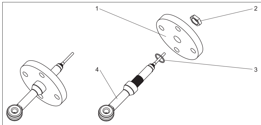
Fixed flange, in contact with medium (order option "process connection": 3, 4)
