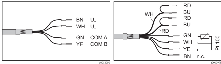
CYK81 for cable extension for CLS50D – max. total cable length: 100 m (330 ft)
