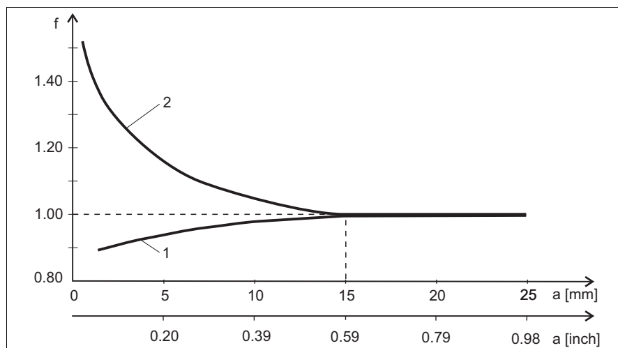
Relationship between installation factor f and distance from wall a
