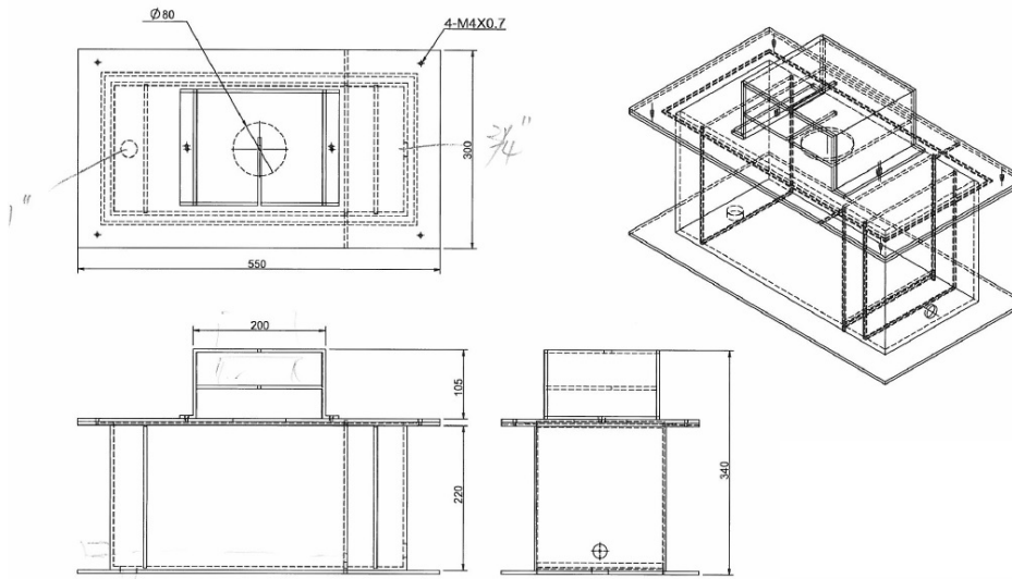
✂Illustration of the flow-through chamber
