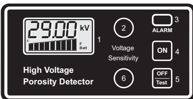
CONTROL LAYOUT
