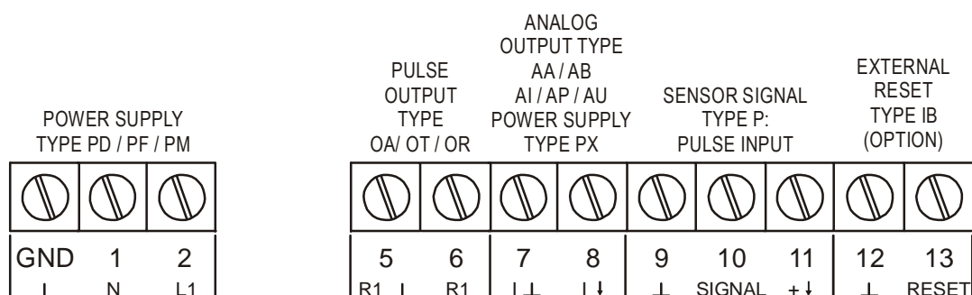
Fig. 9: Overview of terminal connectors standard configuration Gx110P and options.
