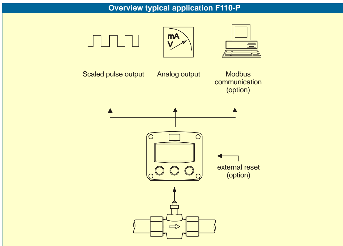
Fig. 1: Typical application for the Gx110P.
