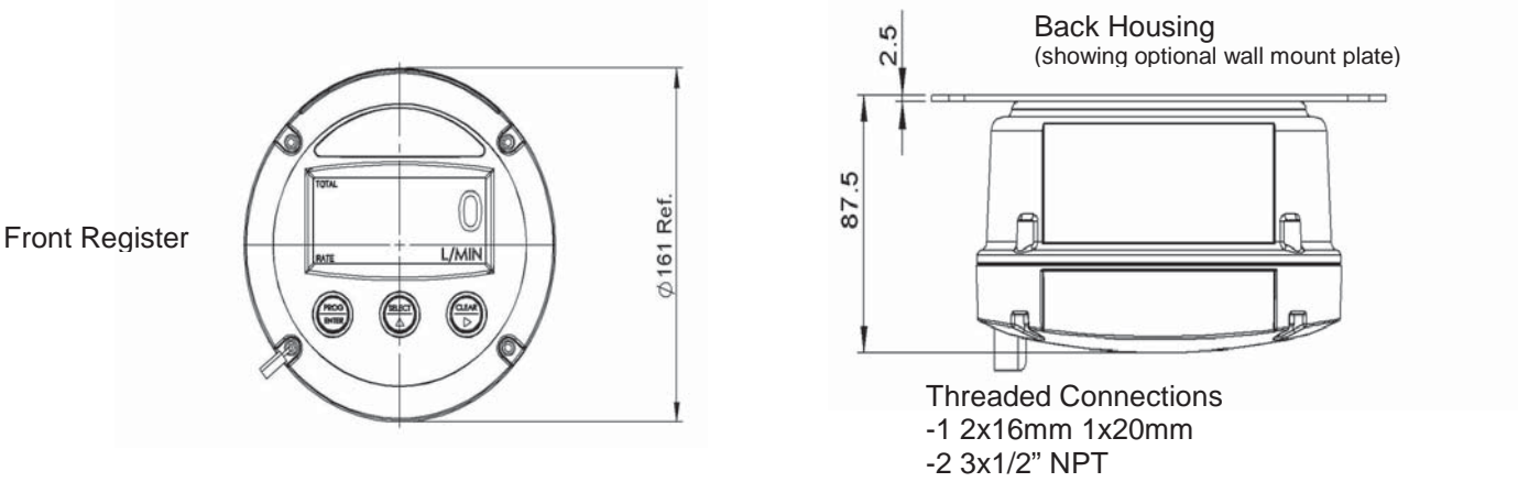
Fig. 6a: Dimensions ER Series meter mount enclosures
