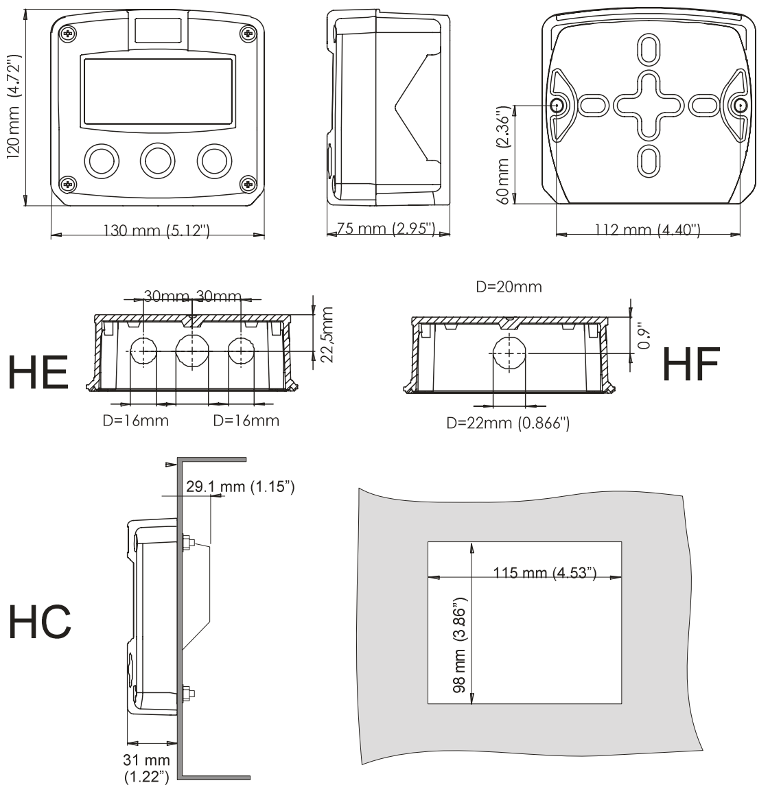
Fig. 8: Dimensions GRP enclosures.
