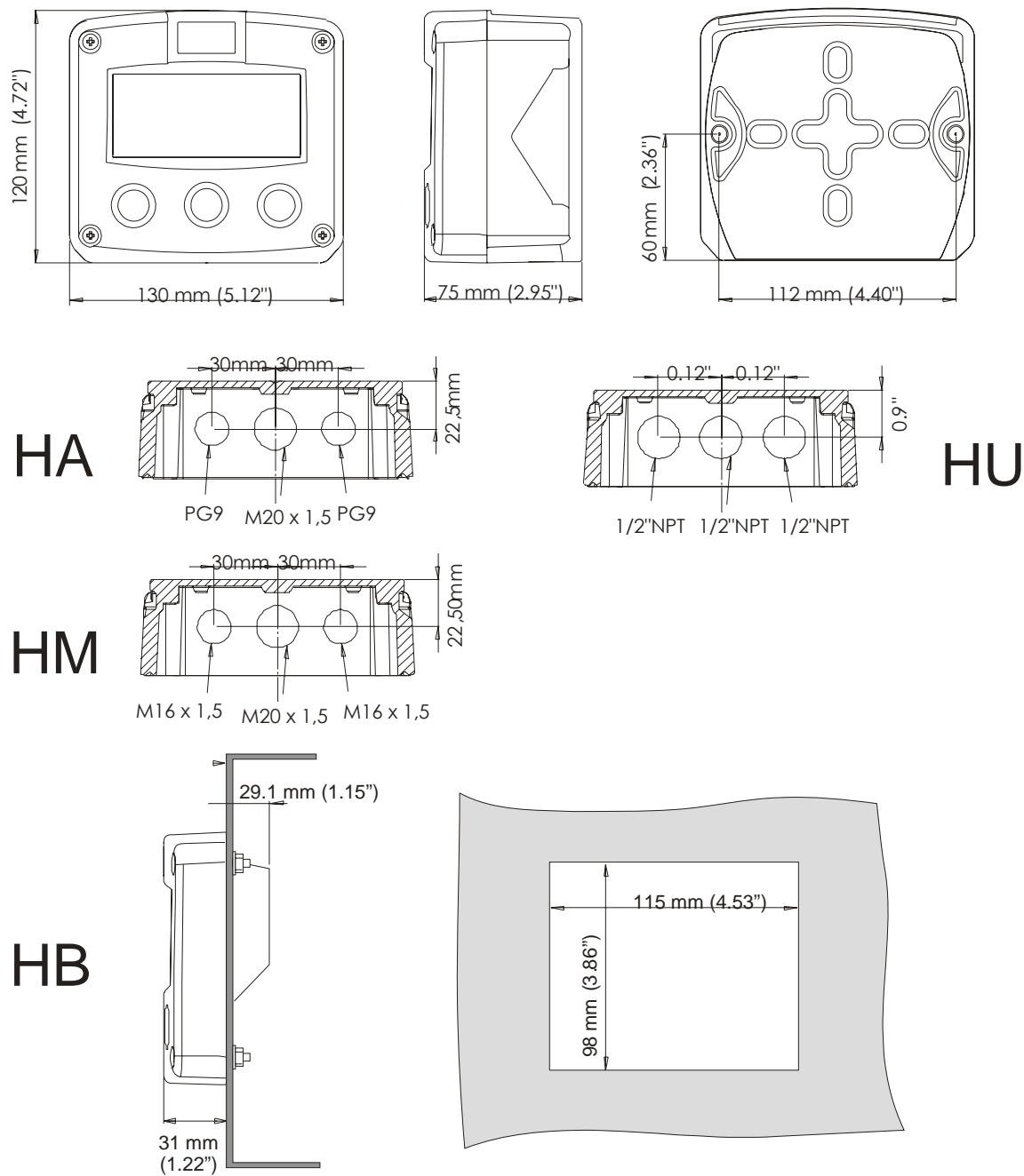
Fig. 7: Dimensions Aluminum enclosures.
