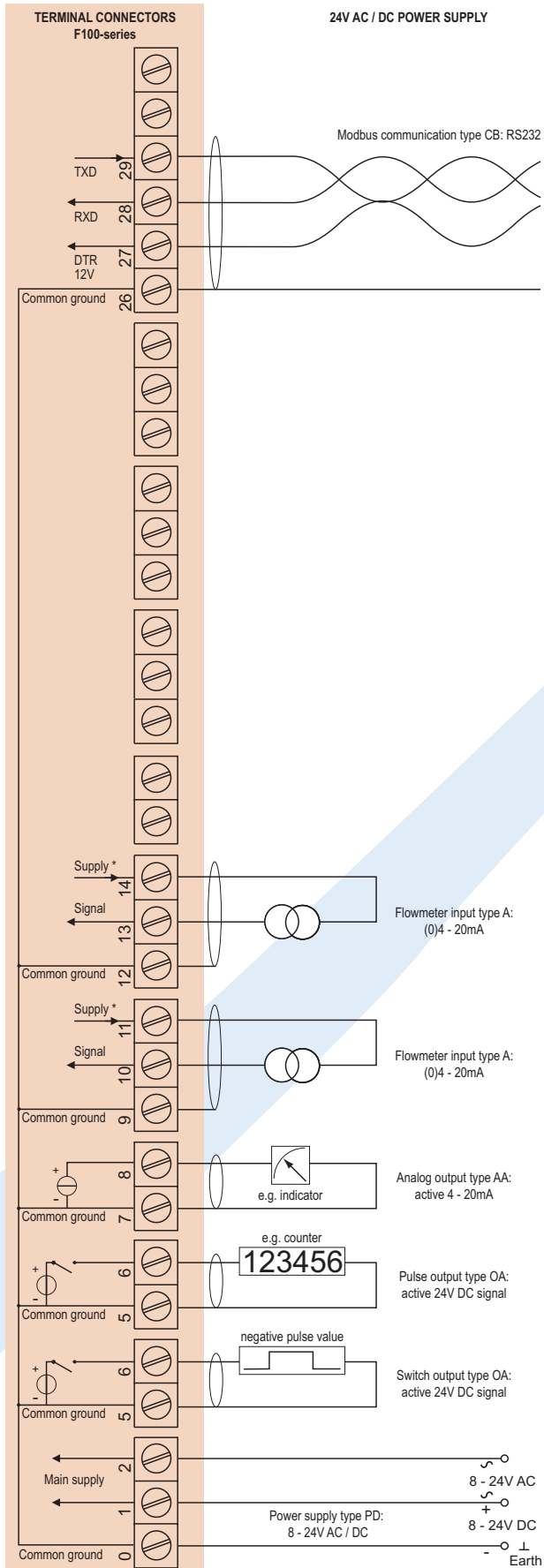
Typical wiring diagram 116-A-AA-CB-OA-PD
