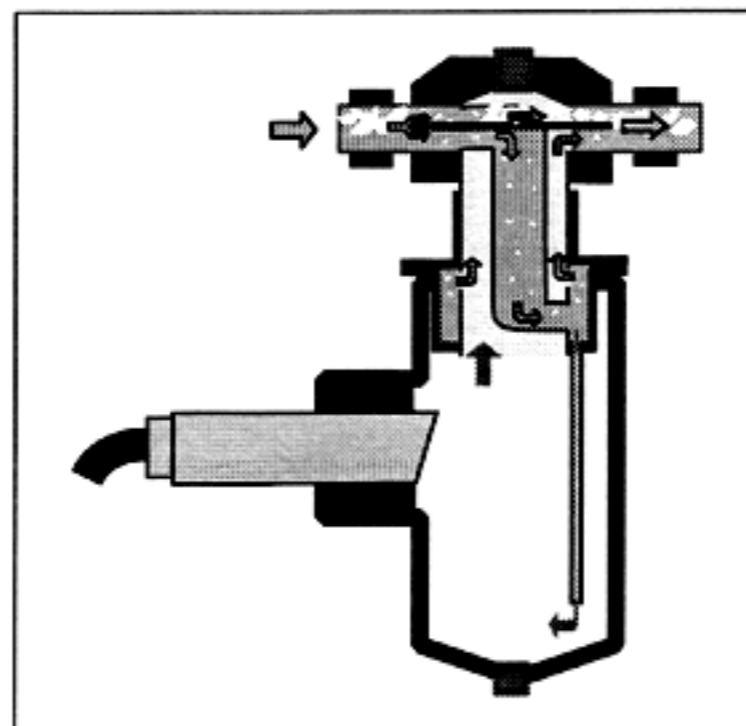
Integrated gas bubble elimination
