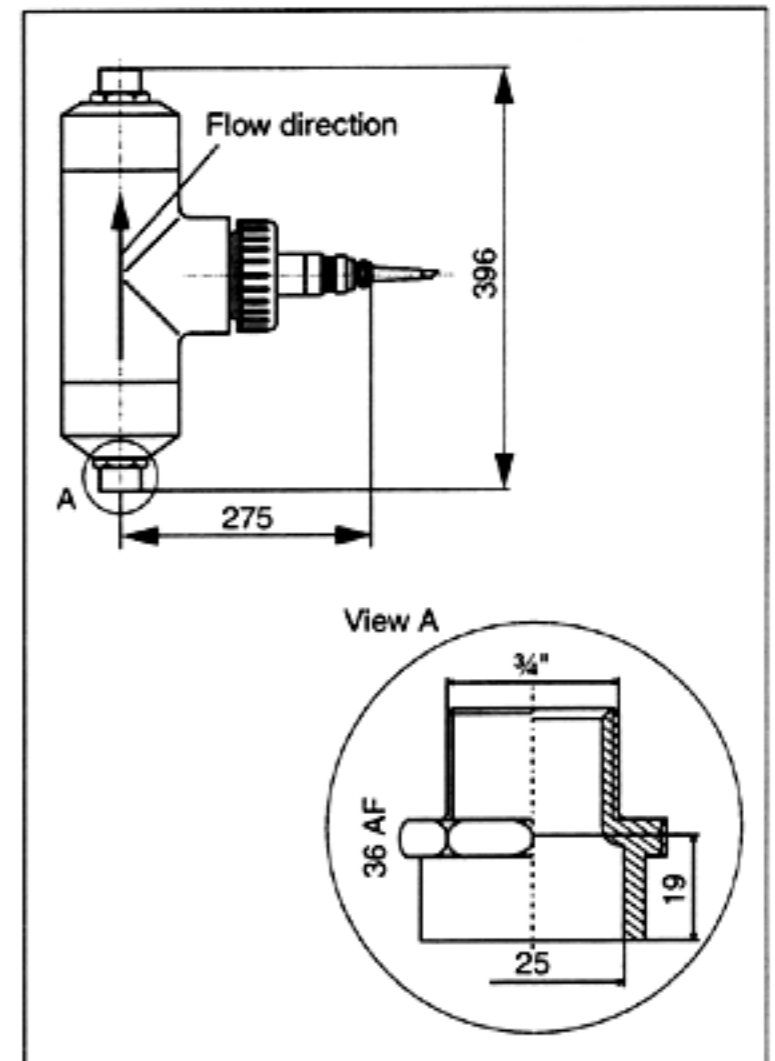
Flow assembly E
