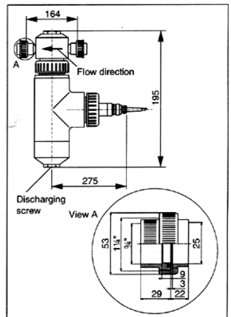
Flow assembly S
