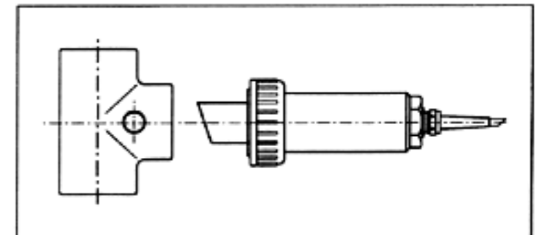
Installed against the medium flow
