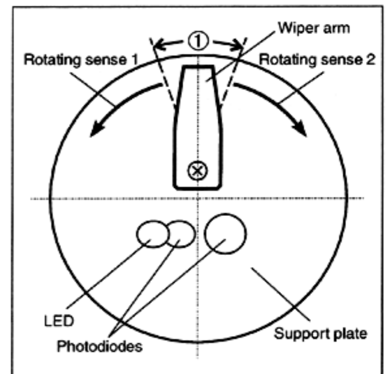
① Rest position of the wiper arm Tolerance range: \pm 20^\circ
