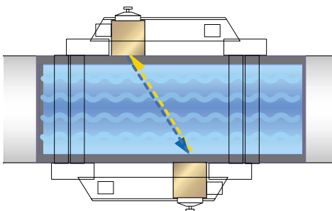
Externally mounted non-wetted sensors (Z-Shot)
