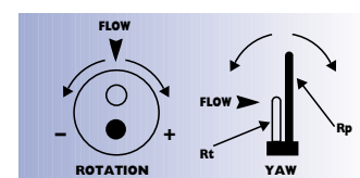
Sensor Rotation and Yaw Description.
