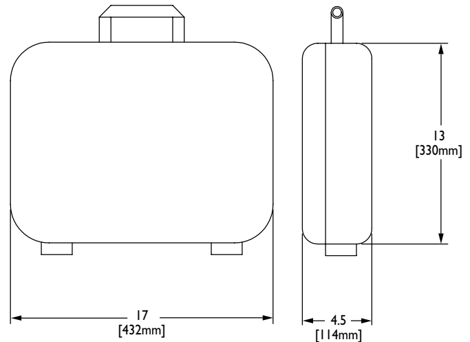
Model 2443 Carrying Case
