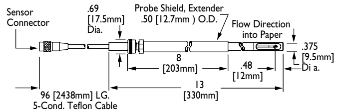
Probe Assembly Shown with Probe Shield
