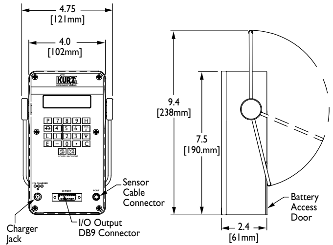
Series 2443 Display Module
