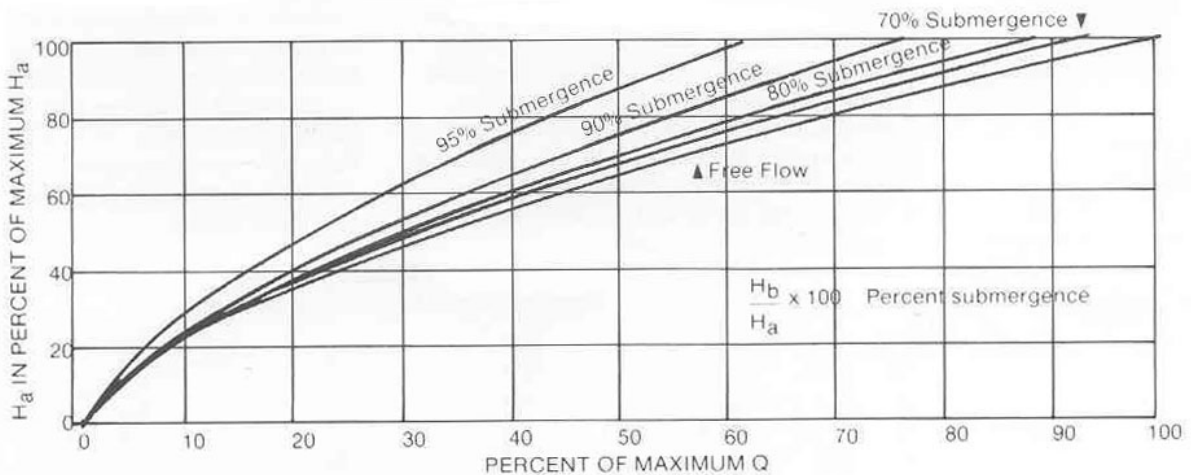
Discharge curves for Parshall flumes with free flow and with submerged conditions.
